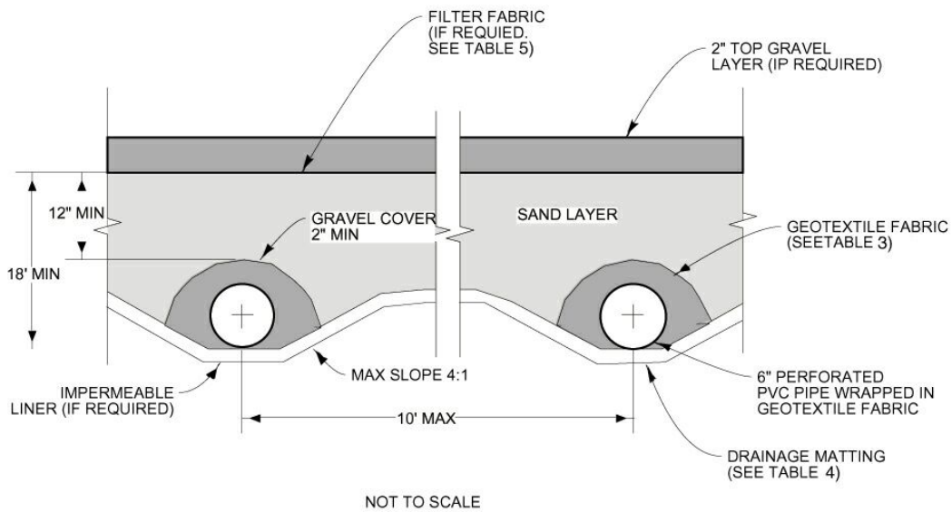
Figure 9B: Filter Bed with Trench Underdrain
