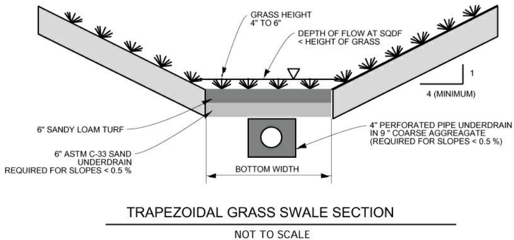
Figure 11: Grassed Swale
