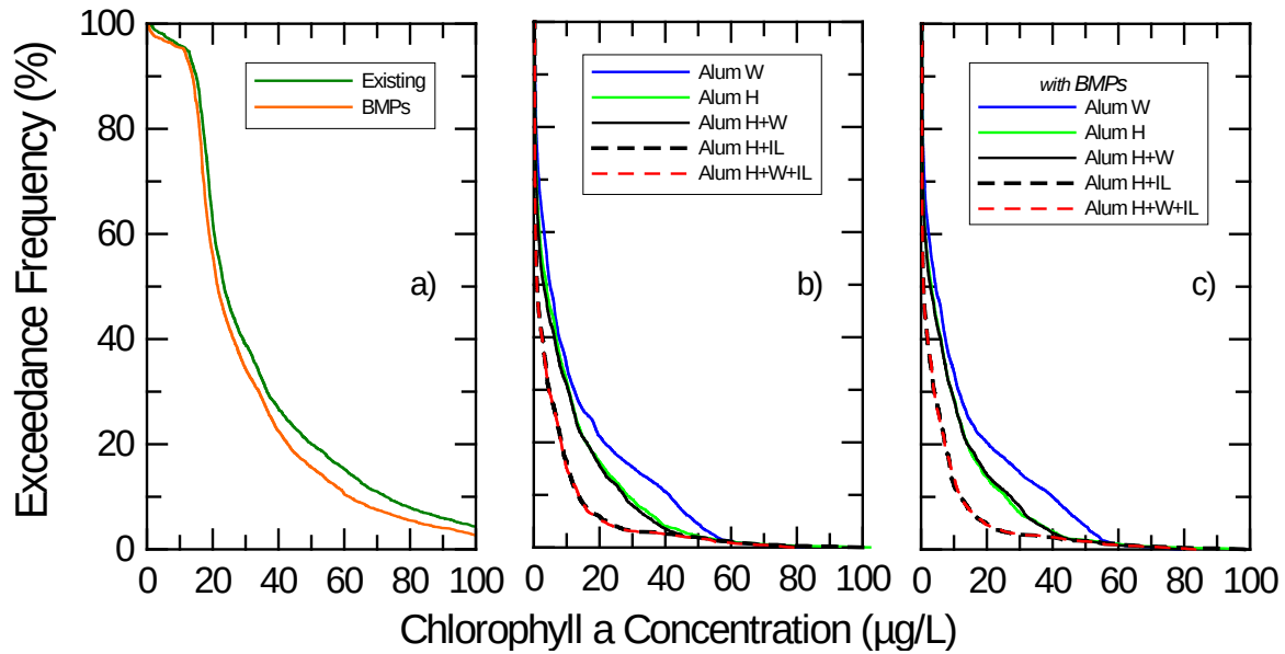
Fig. 7. Cumulative distribution functions showing exceedance frequency as function of simulated chlorophyll a concentrations in Canyon Lake under (a) existing and BMP scenarios, (b) alum treatments, and (c) BMPs with alum treatments.
