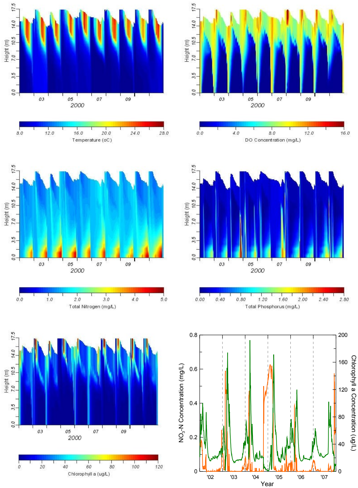
Fig. 7. Predicted water column conditions and water quality in Canyon Lake under reference scenario: a) temperature, b) DO, c) total N, d) total P, e) chlorophyll a, f) NO 3 +chlorophyll a.
