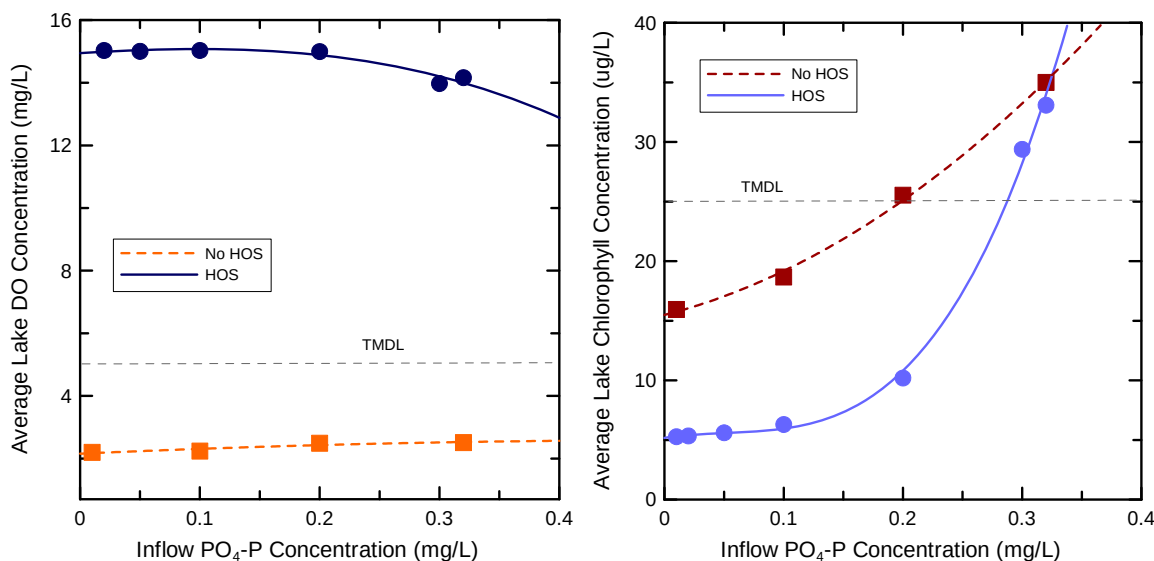
Fig. 6. Predicted average lake concentrations of (a) dissolved oxygen (1 m above bottom) and (b) chlorophyll a as a function of inflow PO 4 -P concentrations.
