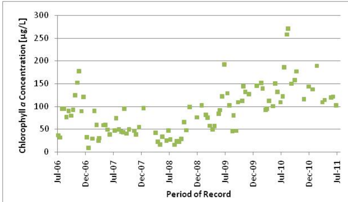
Figure B-10 Lake Elsinore Chlorophyll a Concentrations
