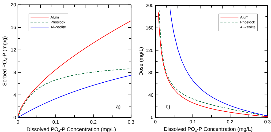
Fig. 1. Comparison of (a) \text{PO}_4\text{-P} adsorption isotherms and (b) treatment doses and corresponding equilibrium dissolved \text{PO}_4\text{-P} concentrations for liquid alum, Phoslock and Al-zeolite (Aqual-P).
