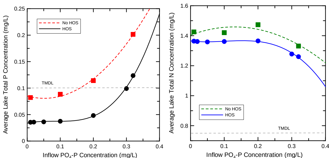
Fig. 5. Predicted average lake concentrations of (a) total P and (b) total N as a function of inflow \text{PO}_4\text{-P} concentrations.
