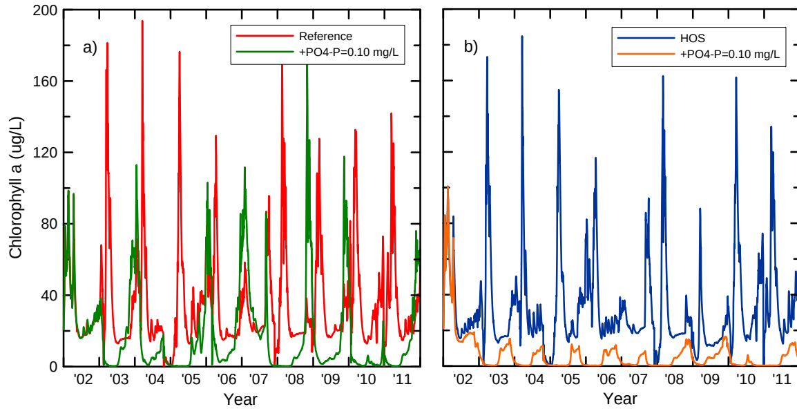
Fig. 4. Predicted chlorophyll a concentrations for (a) the reference scenario and (b) operation of HOS (with and without treatment that reduced inflow \text{PO}_4\text{-P} concentration to 0.10 mg/L).
