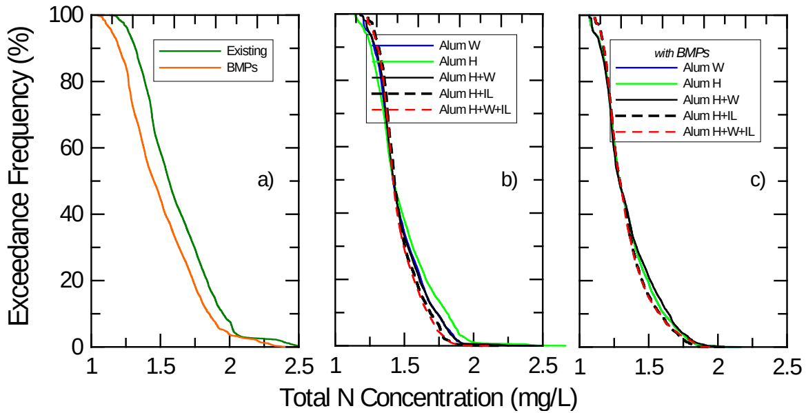
Fig. 6. Cumulative distribution functions showing exceedance frequency as function of simulated total N concentrations in Canyon Lake under (a) existing and BMP scenarios, (b) alum treatments, and (c) BMPs with alum treatments.
