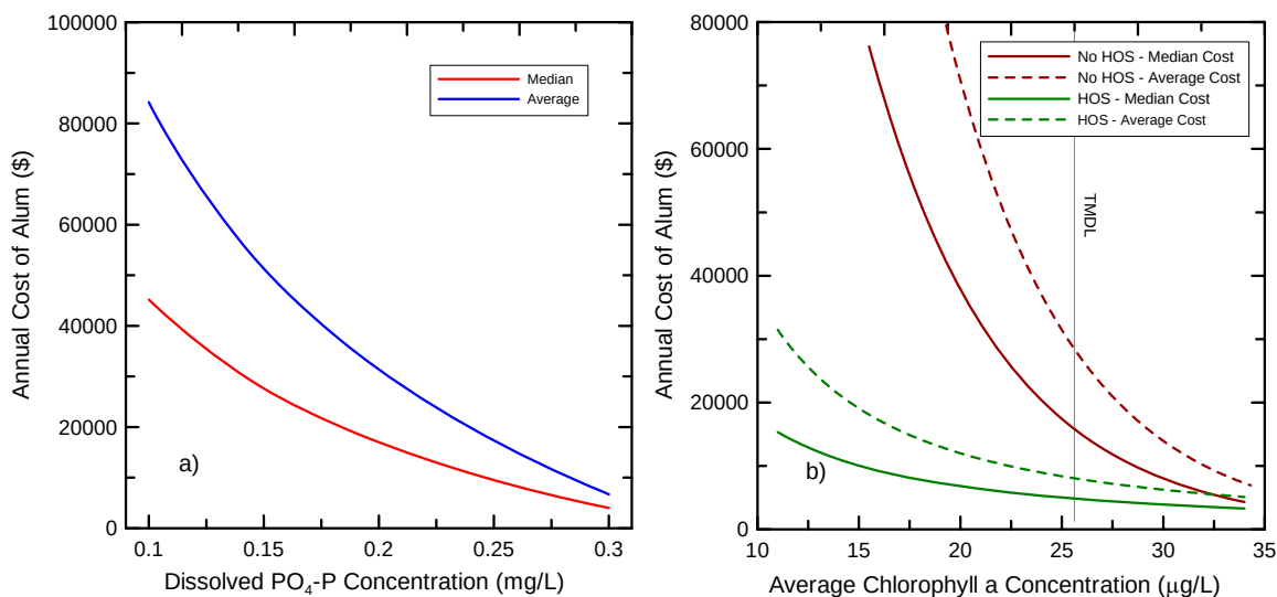
Fig. 7. Projected annual alum costs: a) average and median costs as a function of dissolved \text{PO}_4\text{-P} concentration in inflow to Canyon Lake, and b) median and average costs as a function of chlorophyll a concentration with and without operation of HOS.
